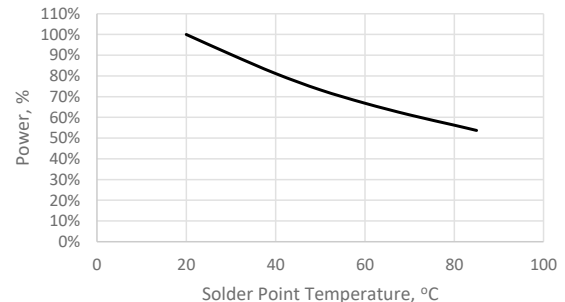
Figure 6. Radiant Flux vs. solder point temperature [ T_a=25^\circ\text{C} , I_f=350\text{mA} ]
