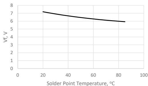
Figure 5. Voltage vs. solder point temperature [ T_a=25^\circ\text{C} , I_f=350\text{mA} ]
