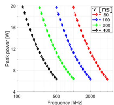
Peak Power at 2040nm vs. Frequency
