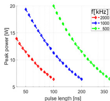
Peak power at 2040nm vs. Pulsewidth
