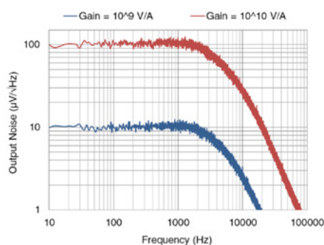
Output Noise
