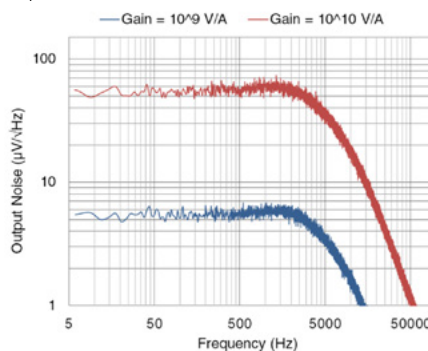
Output Noise
