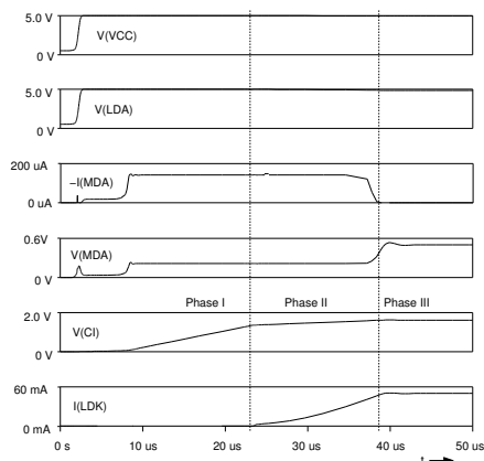
Figure 1: Turn-on behaviour
