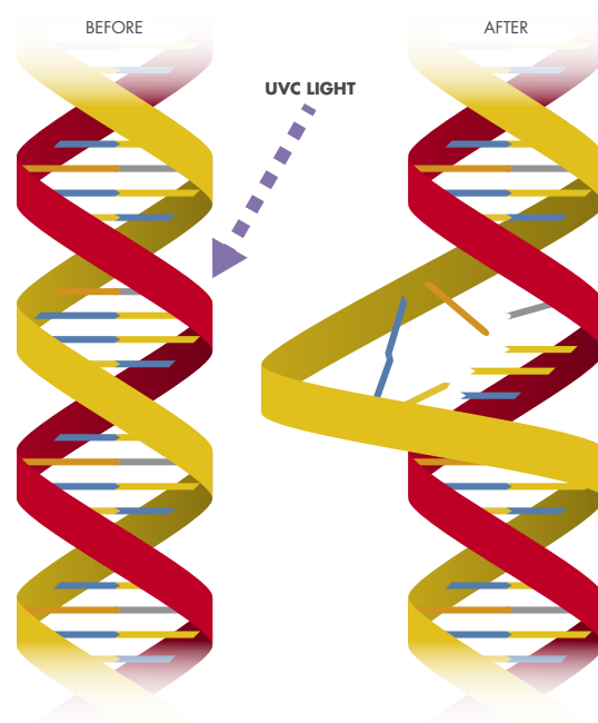
UVC radiation destroys the structure of DNA
